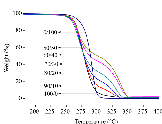
Fig. 9 The TGA curves of PPC and PPC/PBC blends
