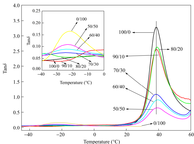
Fig. 2 \tan \delta versus temperature traces of neat PPC, neat PBC, and the PPC/PBC blends
